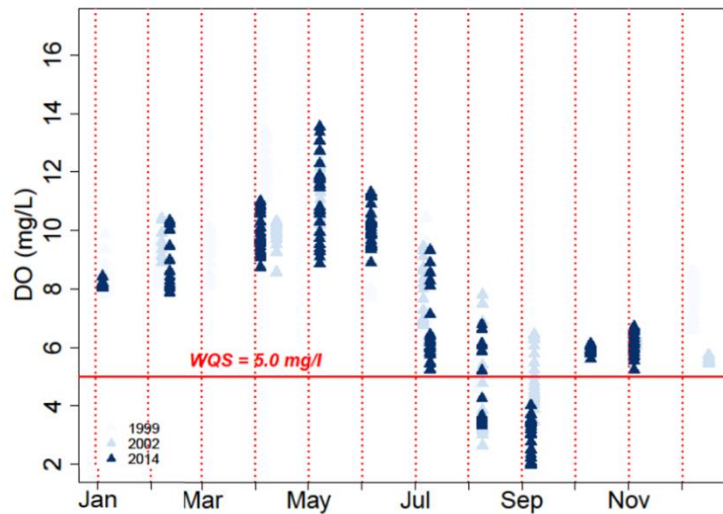
Figure 4.13 DO Concentrations from 1999, 2002, and 2014 at BUD002. Red Line Indicates the 5.0 mg/L Water Quality Criteria for Inner Budd Inlet (Source: Ahmed et al. 2018).
