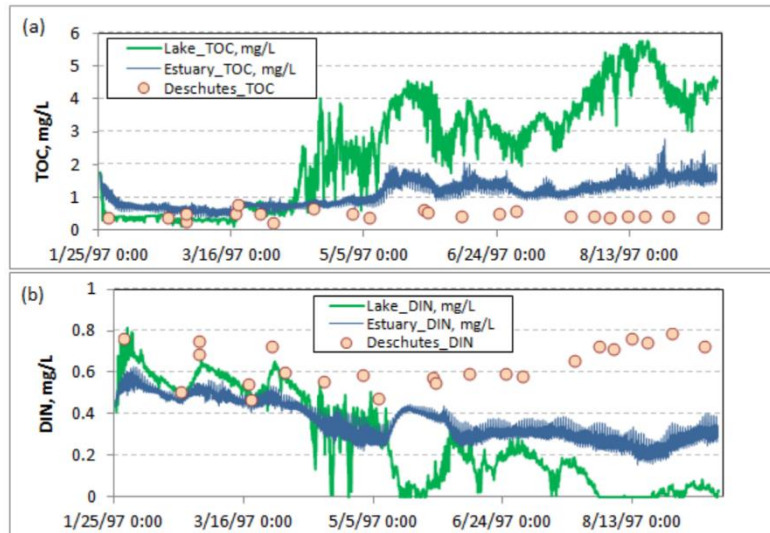
Figure 4.16 Modeled a) Total Organic Carbon (TOC) and b) Dissolved Inorganic Nitrogen (DIN) Concentrations at the Outflow from 5 th Avenue Dam with the Dam (i.e., similar to the Managed Lake Alternative) and Without the Dam (i.e., Estuary Alternative) Compared with Measured Concentrations in the Deschutes River at E Street (Source: Ecology 2015b, Figure 11).
