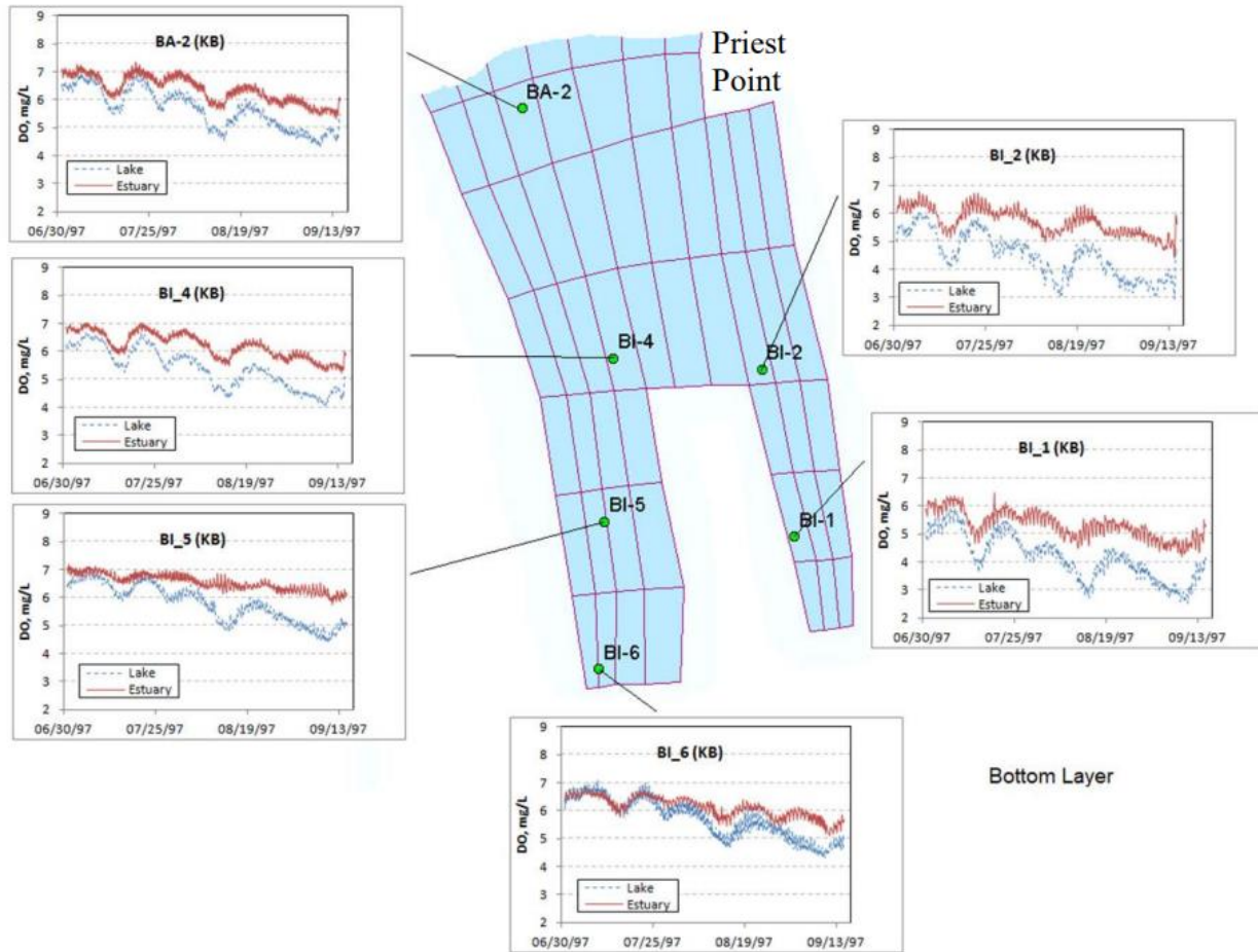
Figure 4.17 Model Predictions of DO in the Bottom Layer at Selected Locations in Budd Inlet Under 1997 Modeled Conditions with Current Anthropogenic Loading With the 5 th Avenue Dam (Blue-Dashed Lines Labeled “Lake”) and Without the 5 th Avenue Dam (Red Line Labeled “Estuary”) (Source: Ecology 2015b, Figure 15).
