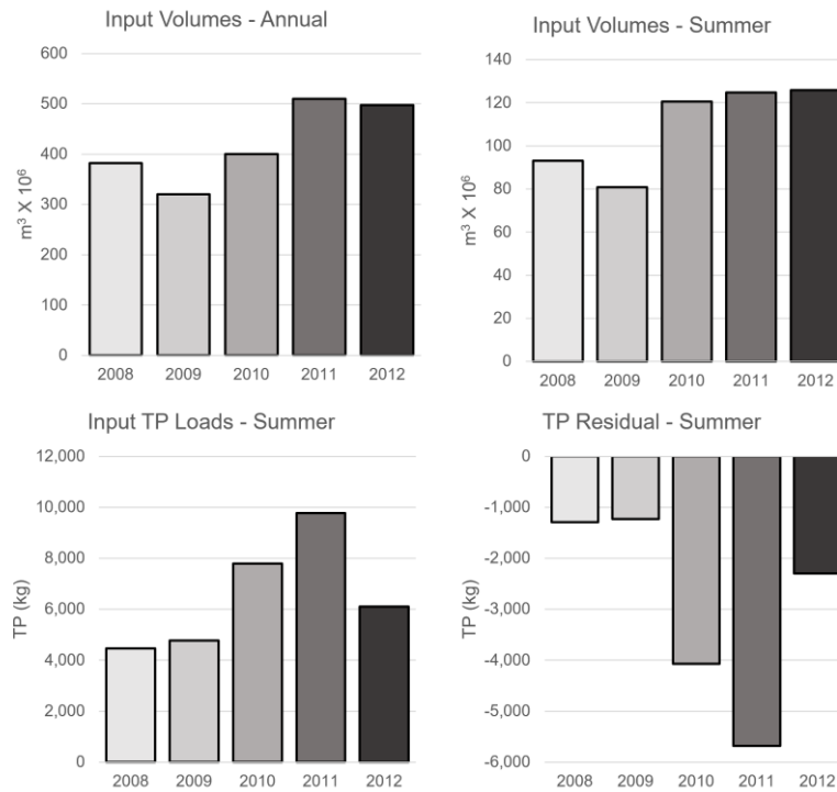
Figure 4.10 Bar Plots of the Annual and Summer Average Input Volumes and TP Loads and Residual TP Load Calculated from the Hydrologic and Phosphorus Budgets by Year.
